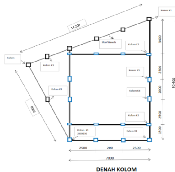
Gambar 3. Denah
